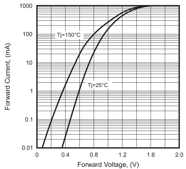
Fig.2 - Forward Characteristics
